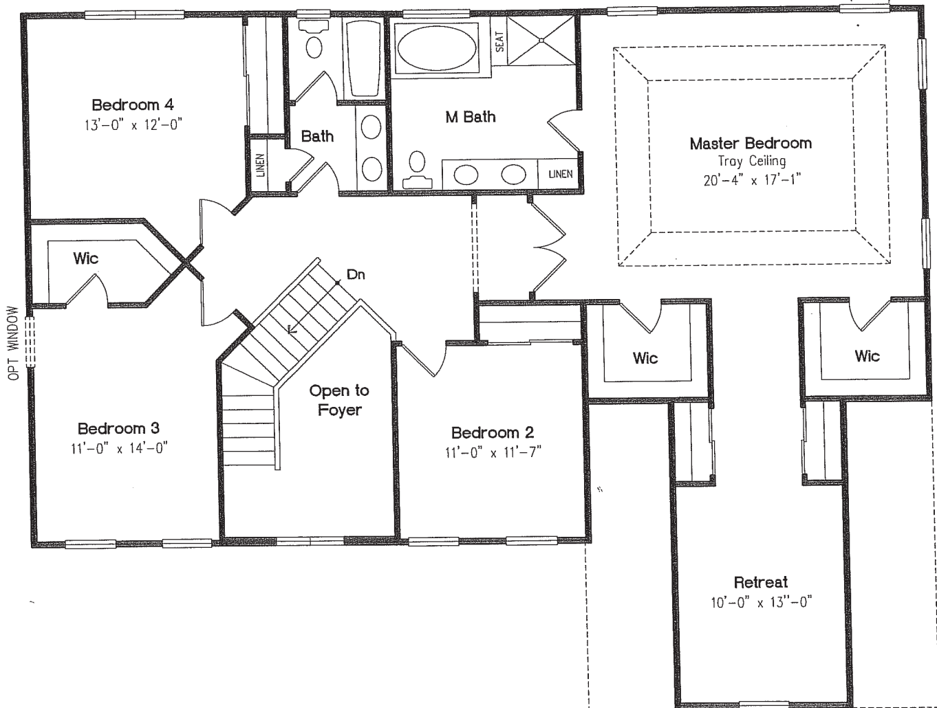
Second Floor Plan - 1607 sf
