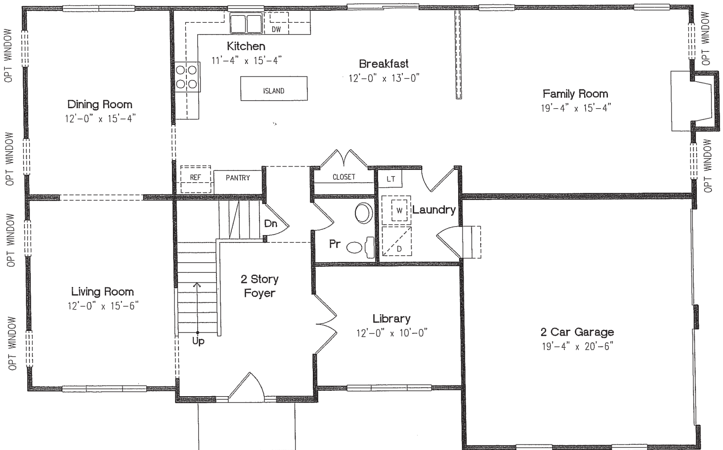
First Floor Plan - 1480 sf
