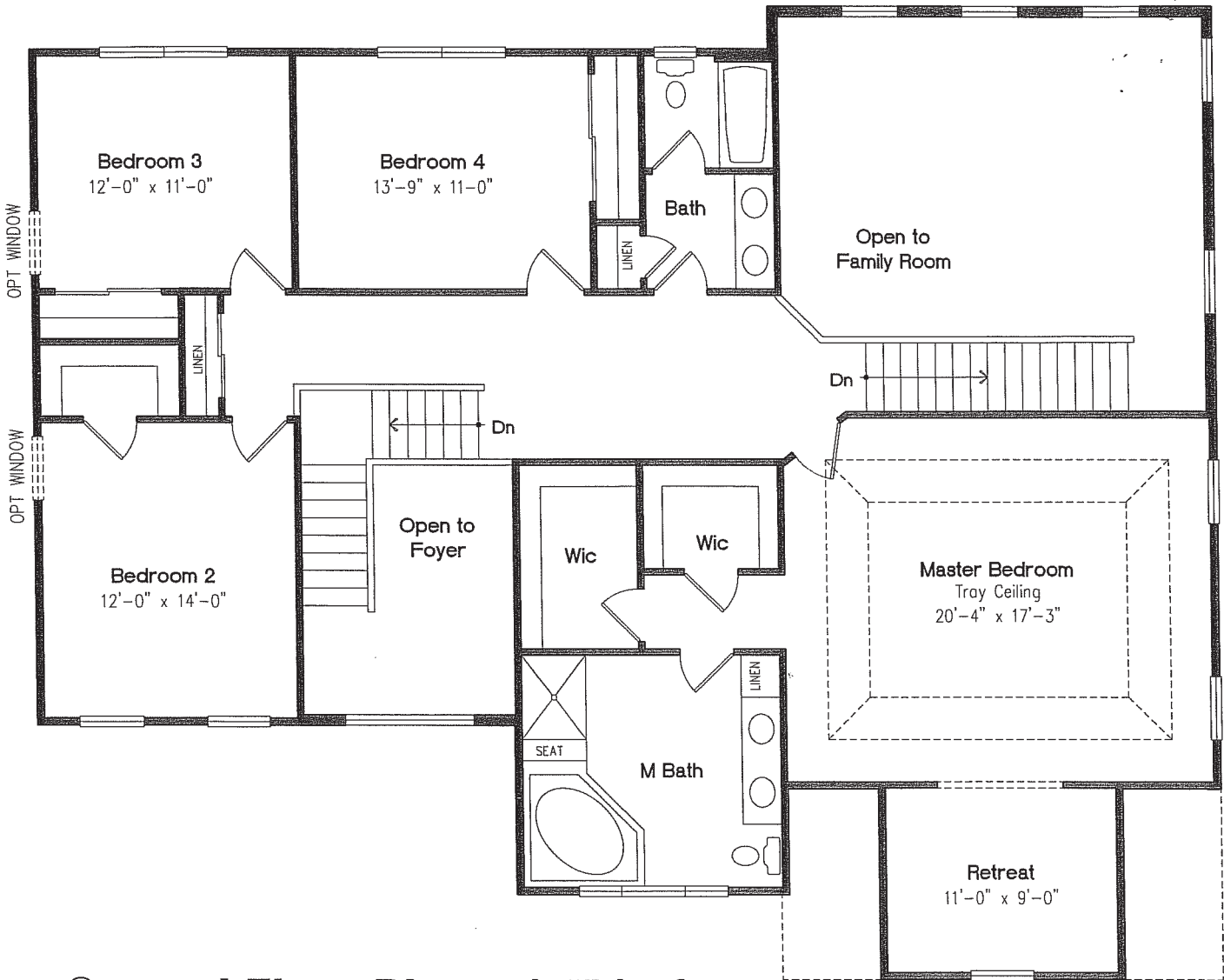
Second Floor Plan - 1571 sf
