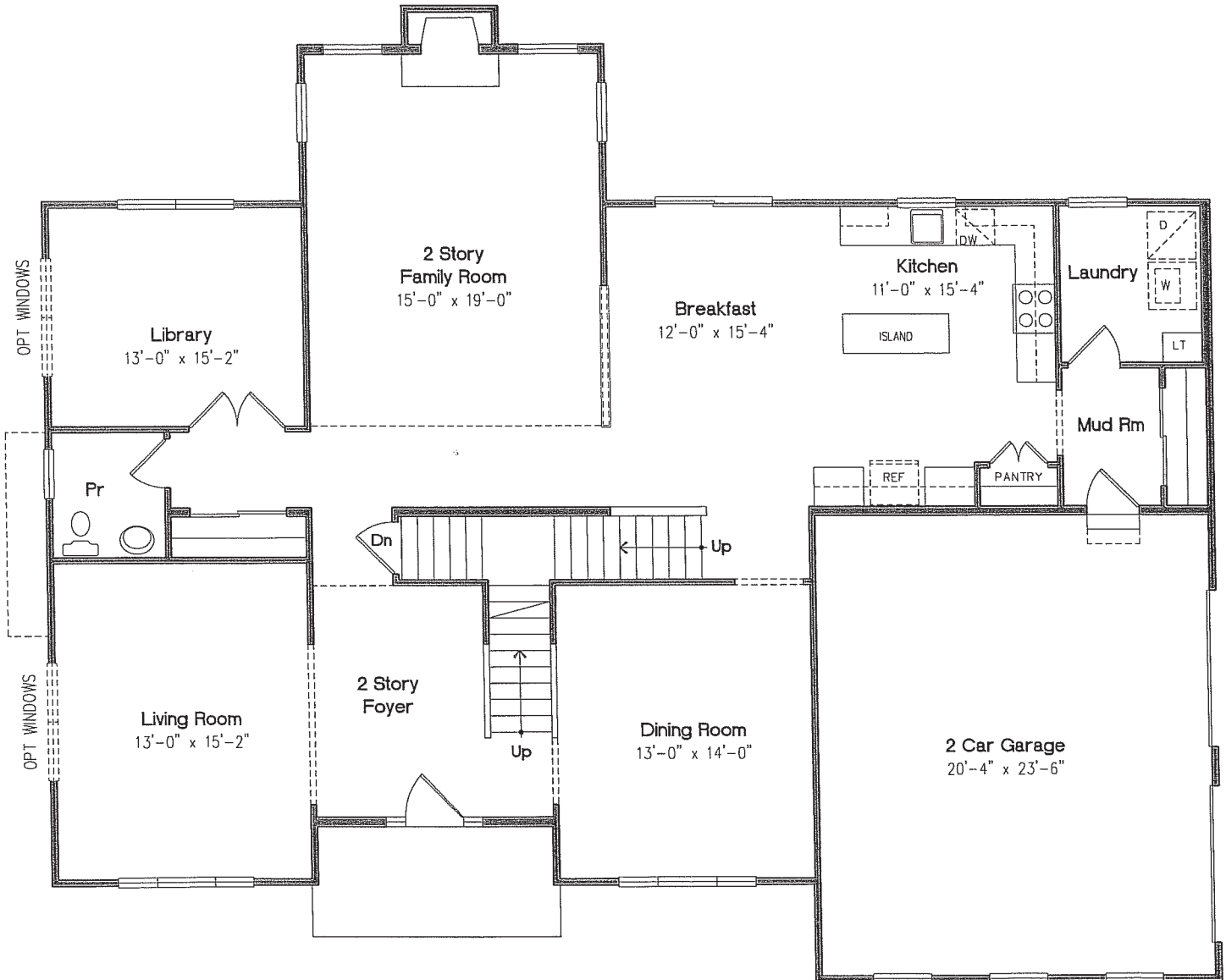
First Floor Plan - 1772 sf
